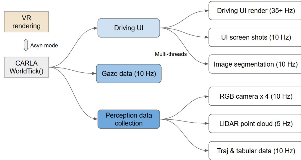
Fig. 14. Architecture of data collection and driving UI built on the CARLA PythonAPI
